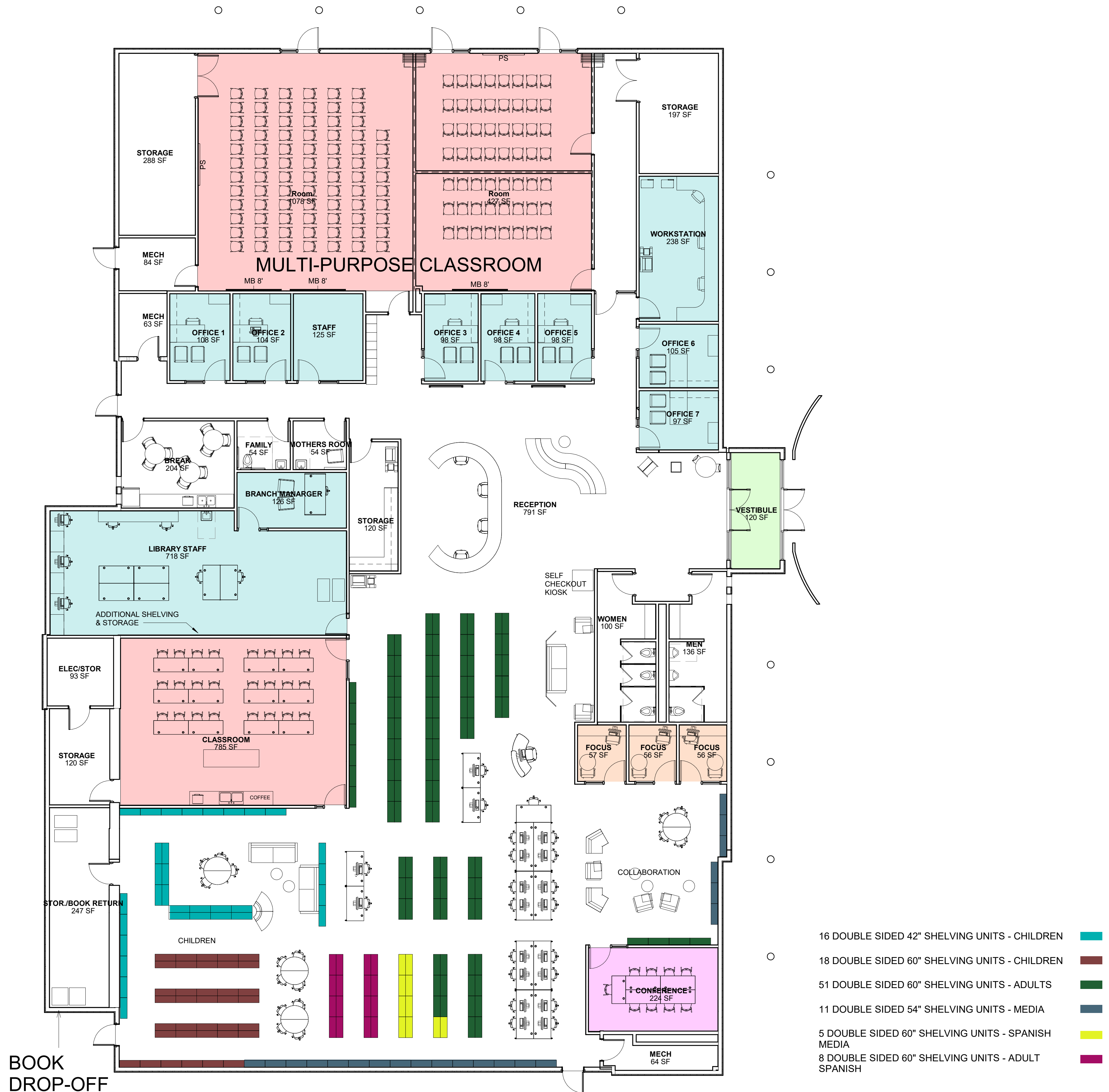
A OPT. 7 - SCHEMATIC FLOOR PLAN - LVL 1 1/8" = 1'-0"
